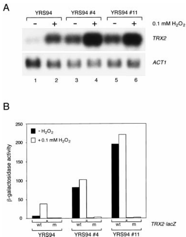
Fig. 2. TRX2 expression in mutants YRS94#4 and YRS94#11. Cultures in early log phase ( OD_{600} = 0.4 ) were split and grown in the absence or the presence of 0.1 mM H 2 O 2 for 30 min. A. Northern blot analysis of total cellular RNA isolated from untreated and treated cells. The experiment was repeated three times, and a representative blot is shown. B. \beta -Galactosidase activity in extracts prepared from untreated and treated cells carrying a wild-type (wt) or mutant (m) TRX2-lacZ fusion. The results shown are from a representative experiment.
