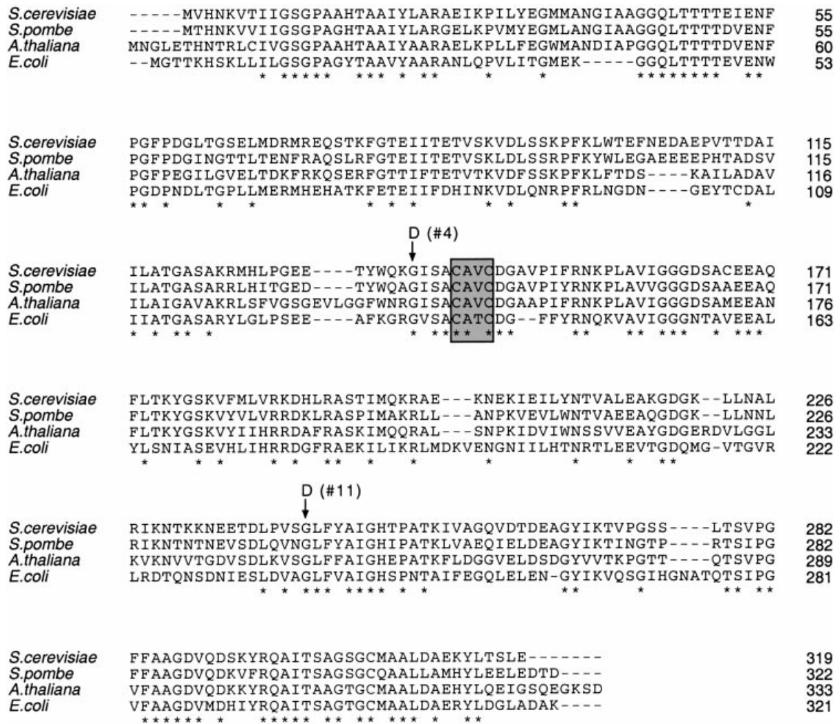
Fig. 3. Position of mutations in YRS94#4 and YRS94#11. The thioredoxin reductase protein sequences of S. cerevisiae (AAB64789), S. pombe (CAA17692), A. thaliana (Q39243) and E. coli (BAA35620) and were aligned using CLUSTAL W (1.8) software. Identical amino acid residues are indicated by the asterisks, the redox-active centre is indicated by the box, and the arrowheads point to the amino acid changes in YRS94#4 (G138D) and YRS94#11 (G243D).
